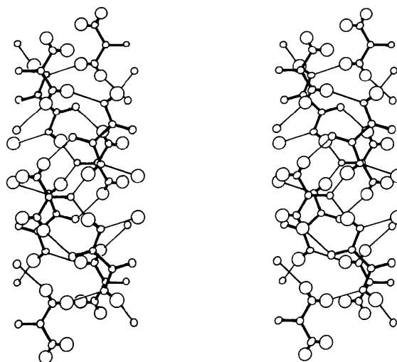
Fig. 2. Stereoview of two parallel planes of urea-oxalic acid (1:1). The viewing direction is perpendicular to (\bar{1}01) . The vibration ellipsoids of the atoms are scaled to include 50% probability.
