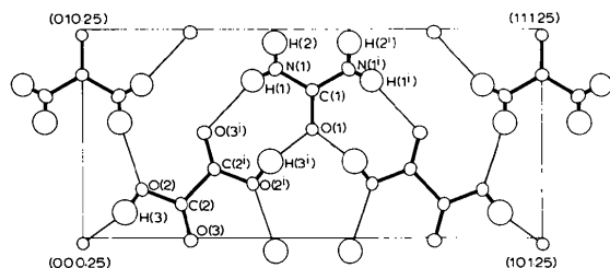
Fig. 1. Projection of the crystal structure of urea-oxalic acid (1:1) on (\bar{1}01) . The vibration ellipsoids of the atoms are scaled to include 50% probability.
